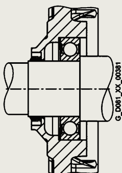
Fig. 4 Drive-end bearing (ZZ Ball Bearing)
