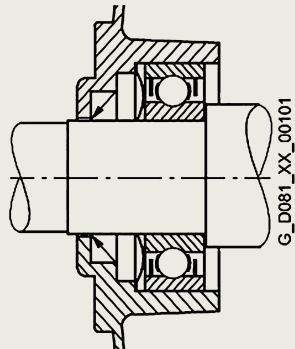
Fig. 2 Drive-end bearing (Re-greaseable Ball Bearing)
