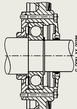
Non-drive end bearing (Re-greaseable Ball Bearing)
