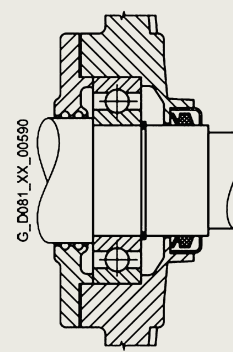
Non-drive end bearing (ZZ Ball Bearing)
