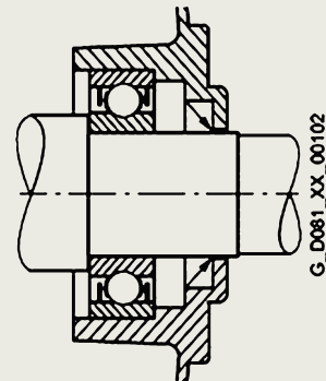
Non-drive end bearing (Re-greaseable Ball Bearing)
